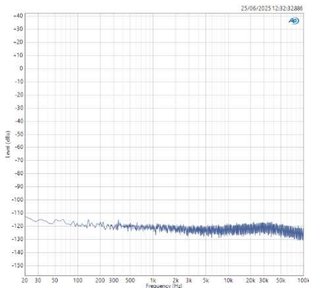
FFT Spectrum Graph – Nagra Compact PSU
